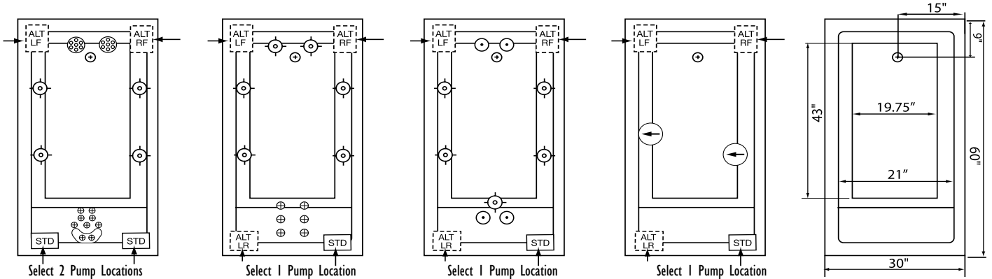
Alt on RH or Alt on LH pump locations will extend past the perimeter of the bath
